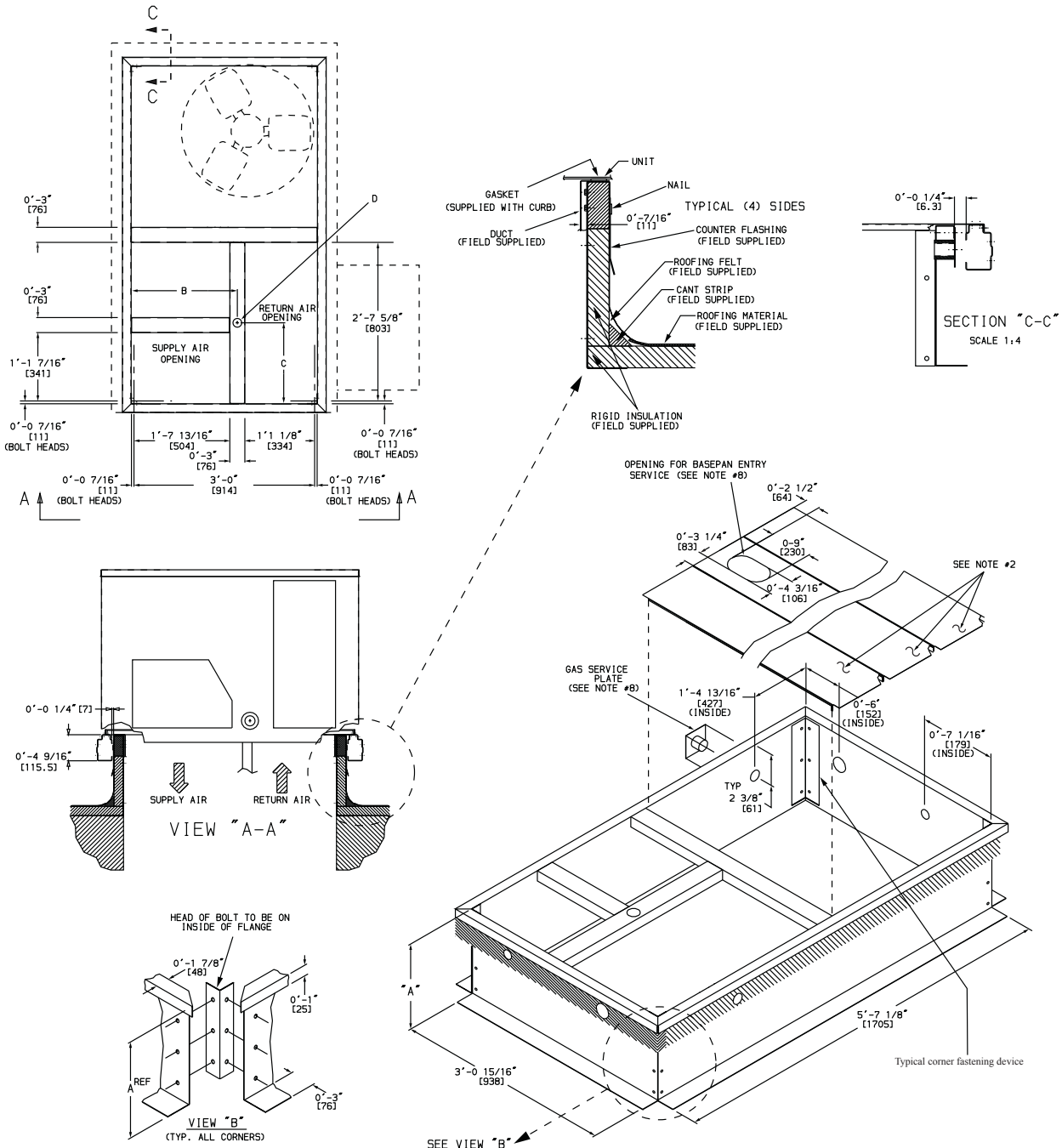
Fig. 4 - Roof Curb Details
