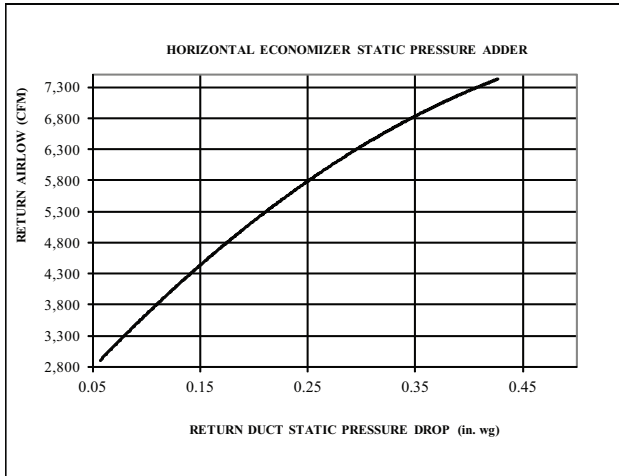
Fig. 20 - Return Air Pressure Drop-Horizontal 15 Ton
