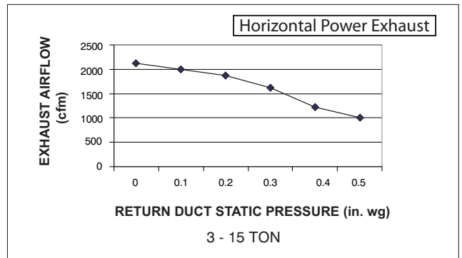
Fig. 23 - Horizontal Power Exhaust Performance
