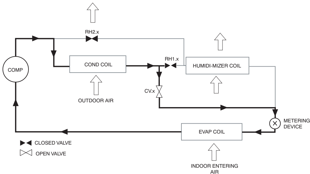
Normal Cooling Mode - Humidi-MiZer System (48TC04-16)
