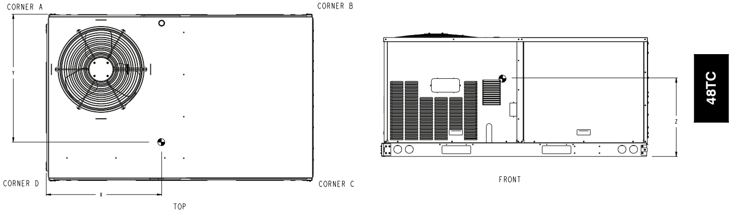
Fig. 2 - Dimensions 48TC 04-07
