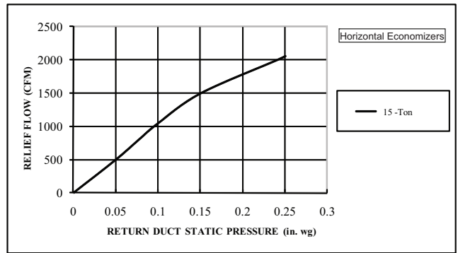
Fig. 22 - Barometric Relief Flow-Horizontal 15 Ton
