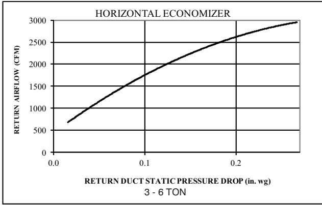
Fig. 18 - Return Air Pressure Drop
