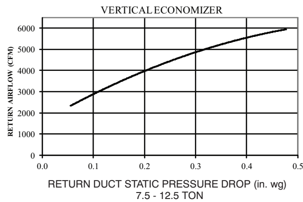
Fig. 13 - Return Air Pressure Drop
