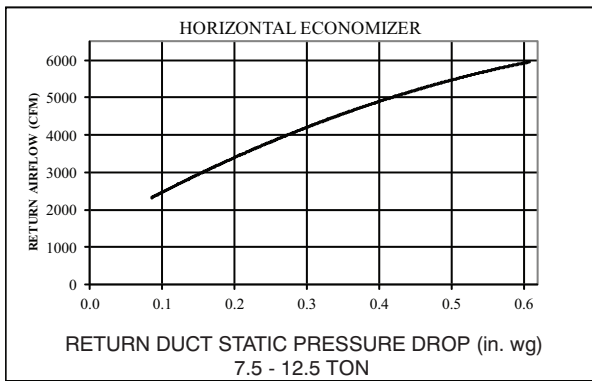
Fig. 19 - Return Air Pressure Drop
