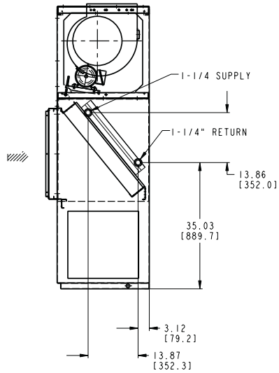
RIGHT SIDE
