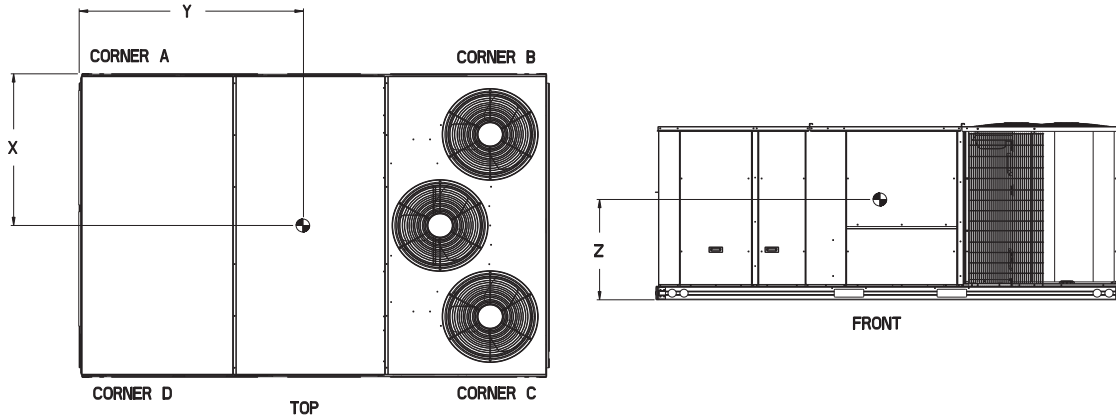
Fig. 2 - Dimensions 50TC-D17-20
