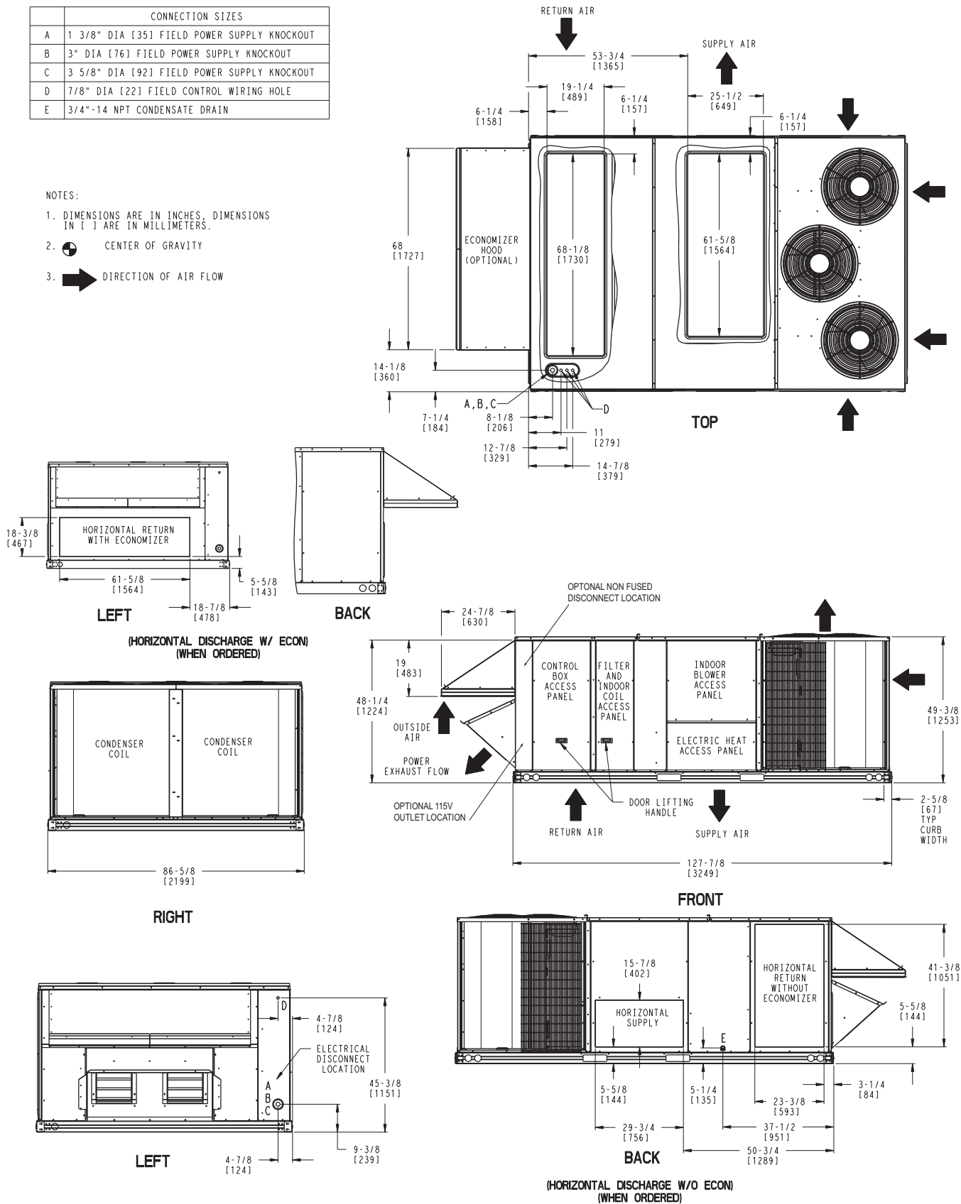
Fig. 1 - Dimensions 50TC-D17-20
