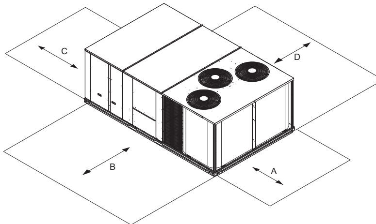
Fig. 3 - Service Clearance
