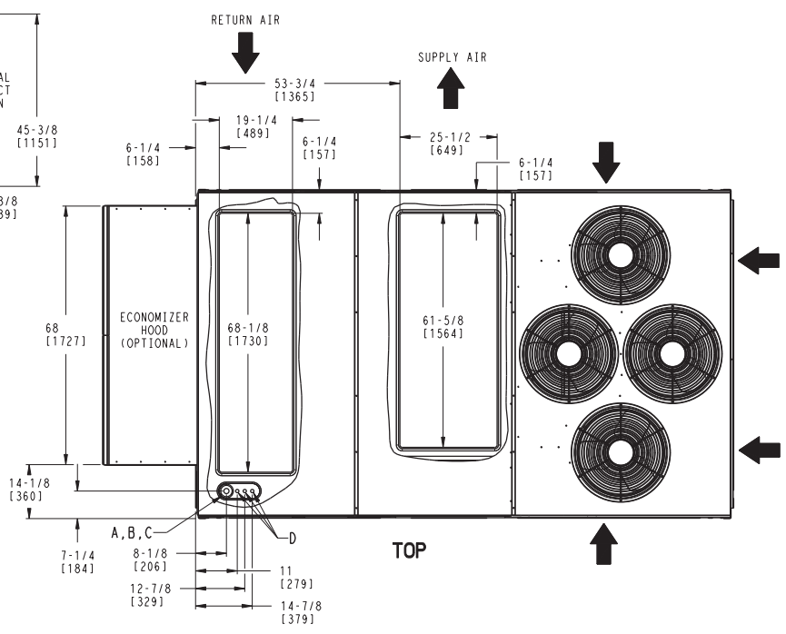
Fig. 5 - Dimensions 50TC-D24-28
