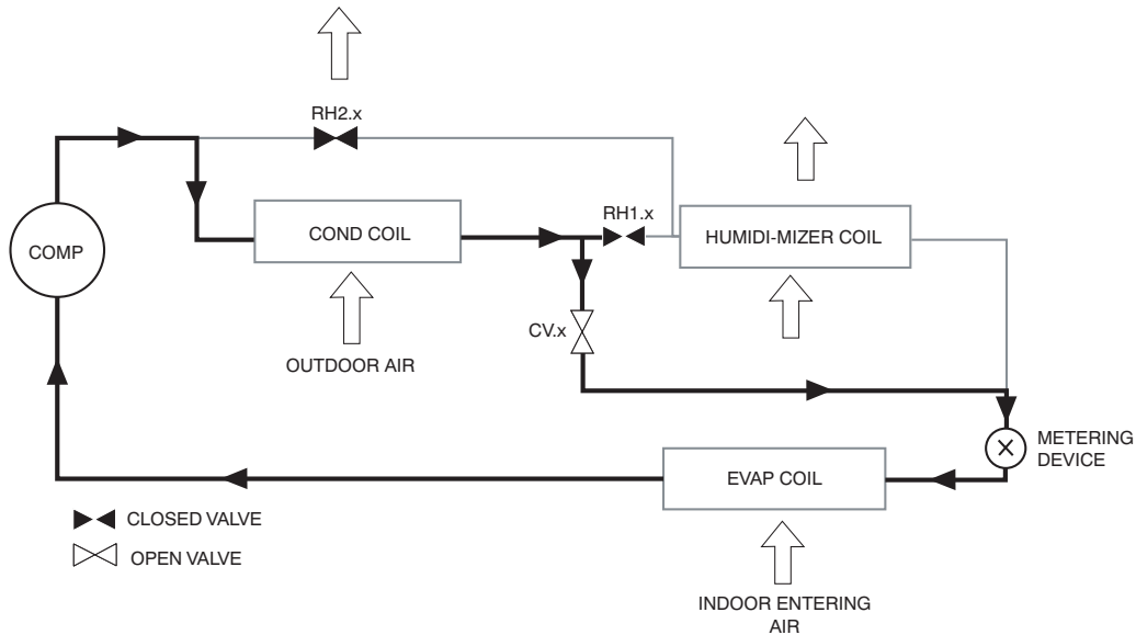
Normal Cooling Mode - Humidi-MiZer System (50TC17-28)
