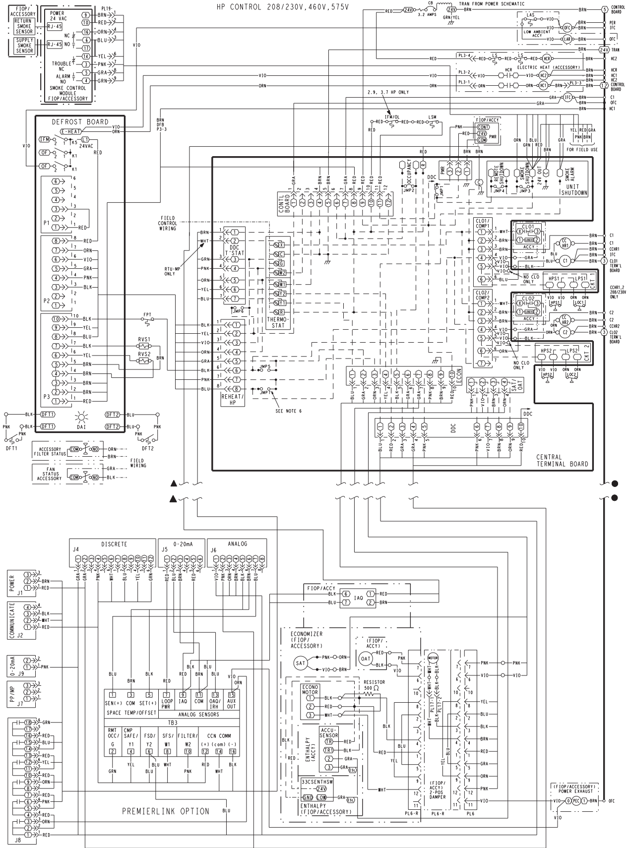
Fig. 14 - PremierLink™ Diagram
