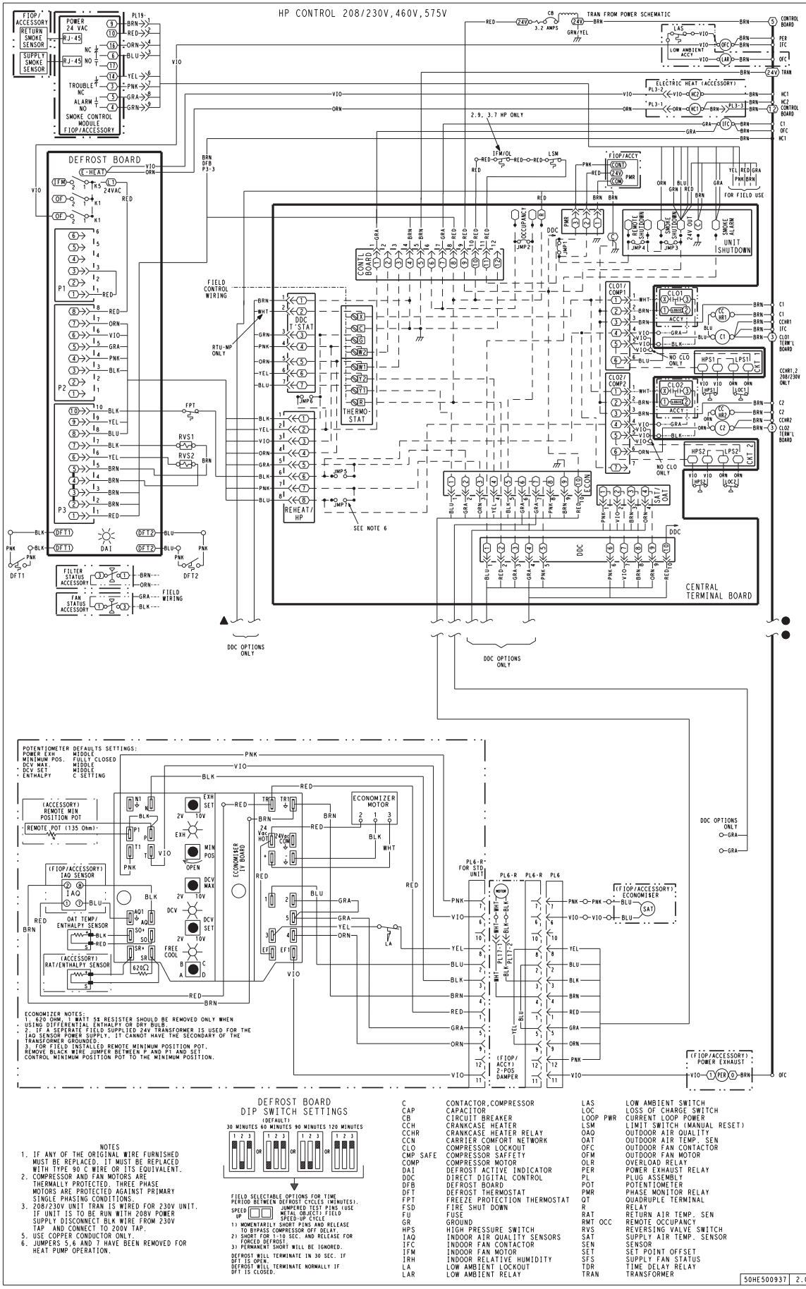
Fig. 13 - Typical Control Diagram
