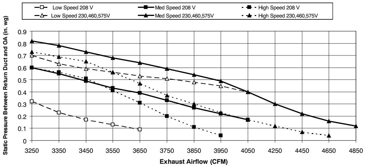
Fig. 11 - Power Exhaust Fan Performance
