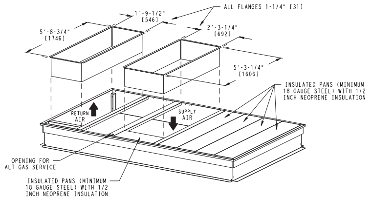
Fig. 8 - Roof Curb Dimensions 50TCQ-24
