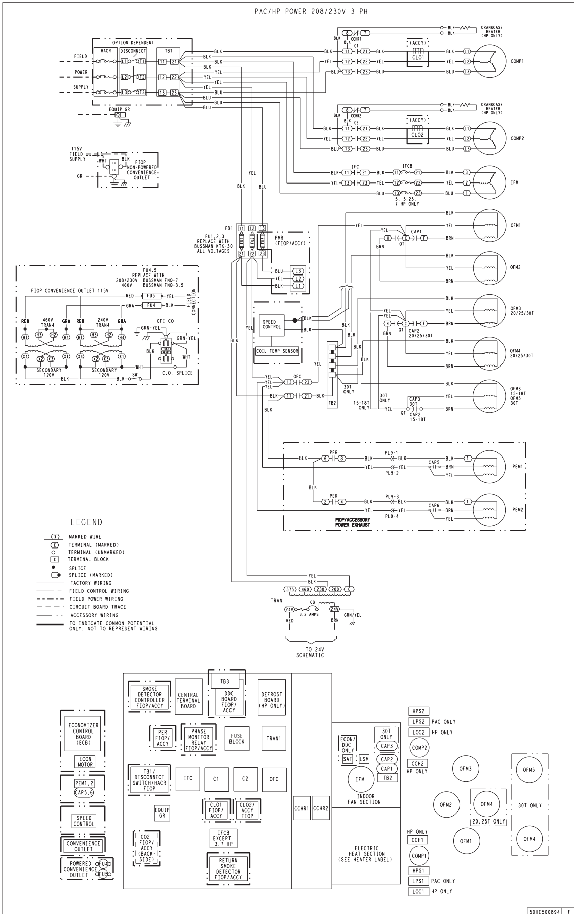
Fig. 12 - Typical Power Diagram
