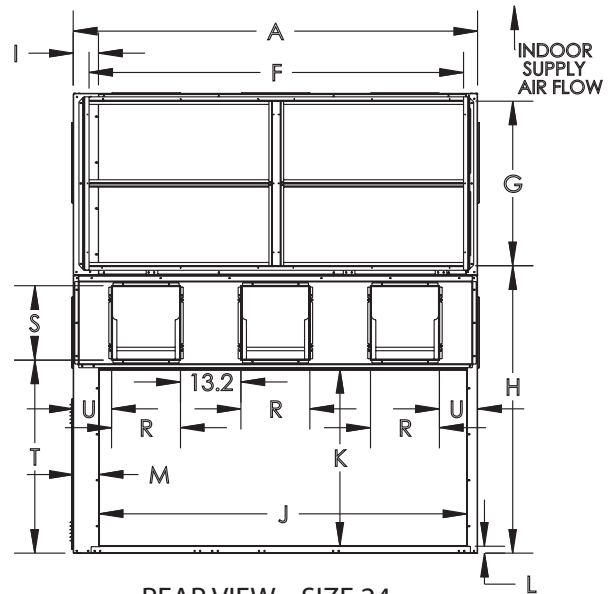
REAR VIEW SIZE 24
