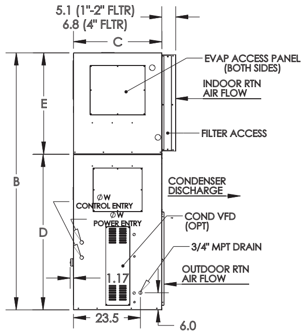
RIGHT VIEW
