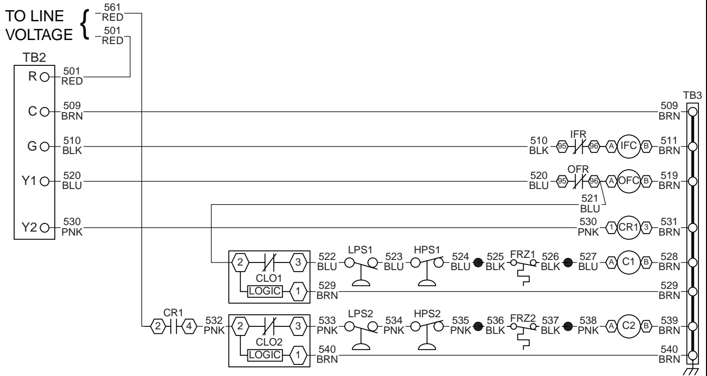
LOW VOLTAGE DIAGRAM — 50XCA012-024, 208/230-3-60 UNITS SHOWN
