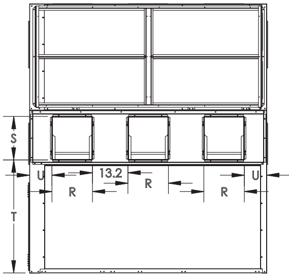
REAR VIEW SIZE 24
