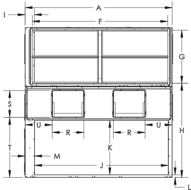
REAR VIEW SIZE 16
