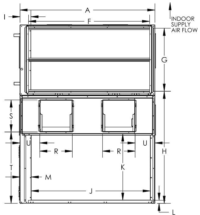
REAR VIEW
