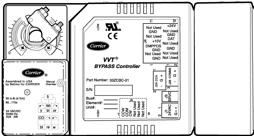
BYPASS CONTROLLER
