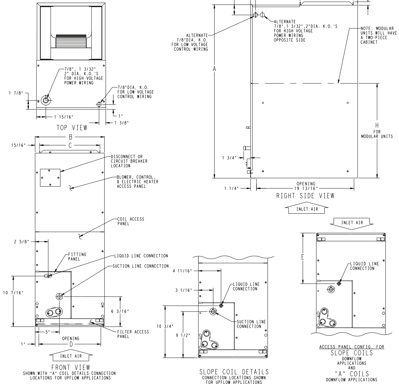
Fig. 1 - FY5B Dimensions - English
